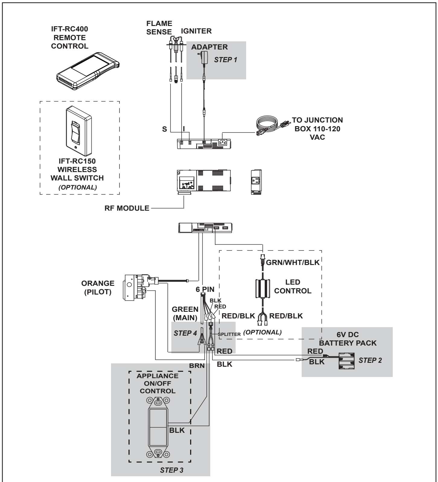
Figure 6 IFT-RC400 Wiring Diagram without SMART-WALL-B
